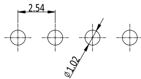
RECOMMENDED PCB LAYOUT (TOLERANCE: ±0.05)
